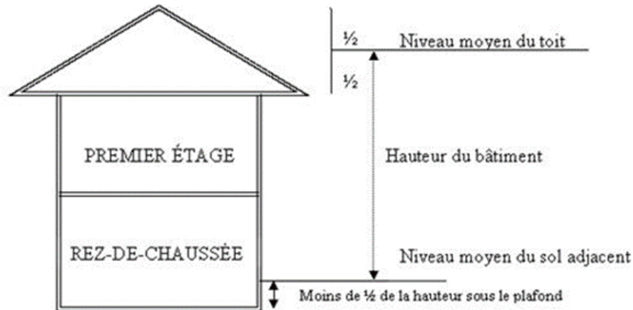
Figure 14 – Rez-de-chaussée
